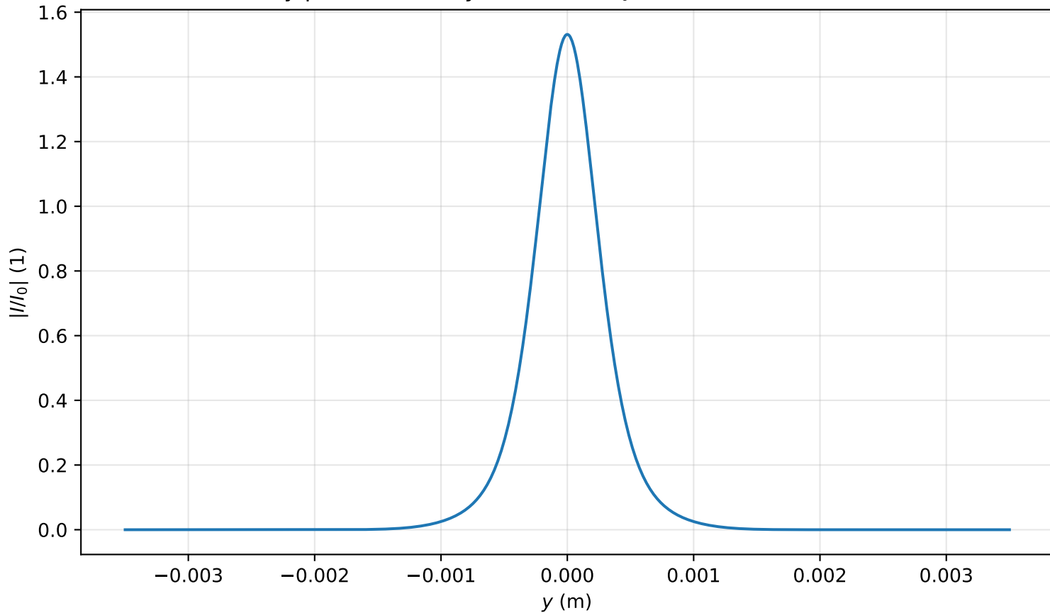
Intensity profile I(x=0, y, z=1.353)/I_0 , P_{in}=0.9P_{cr} , artificial time
